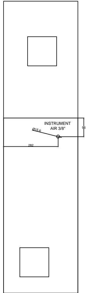
LEFT VIEW TYPE 23 1250 X 750 X 320
